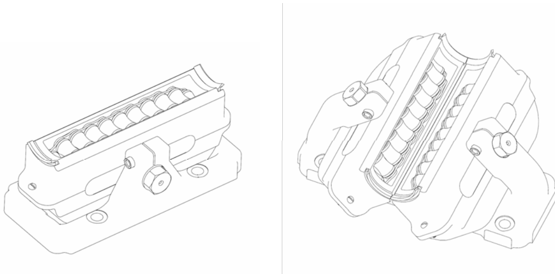
Figure A: Roundway 'S' bearing (left) and Roundway 'V' bearing (right)
