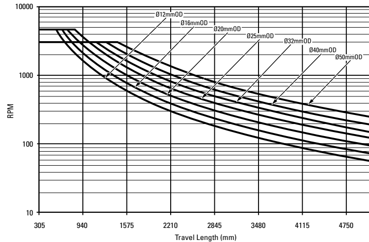
Figure 1 - Critical Speed Graph
